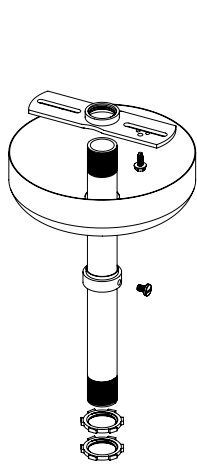
ST12 = 12" Stem (1/2" Dia.) w/ Static Canopy
