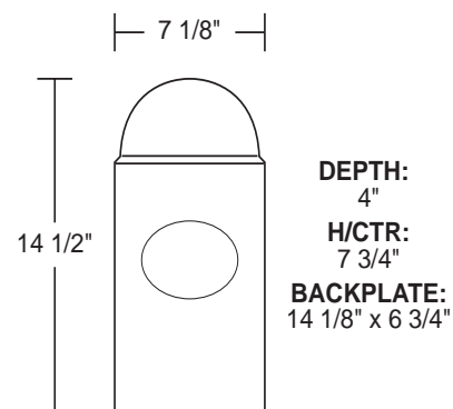
WL101 Dimensions
